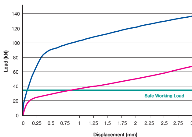
M20 - Connection Load vs Ply Displacement
