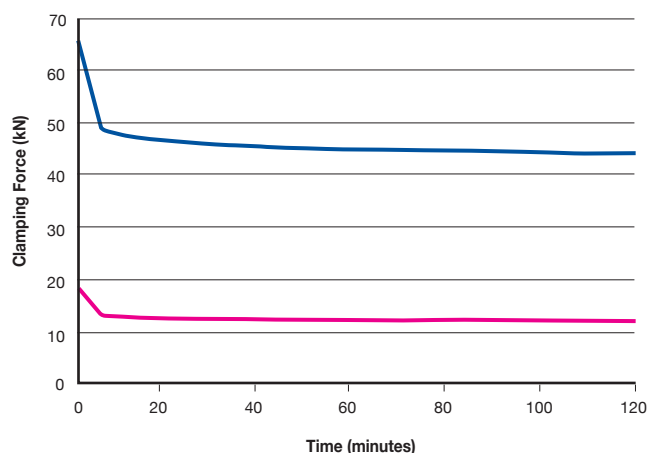
M20: Up to 3.5x Clamping Force
