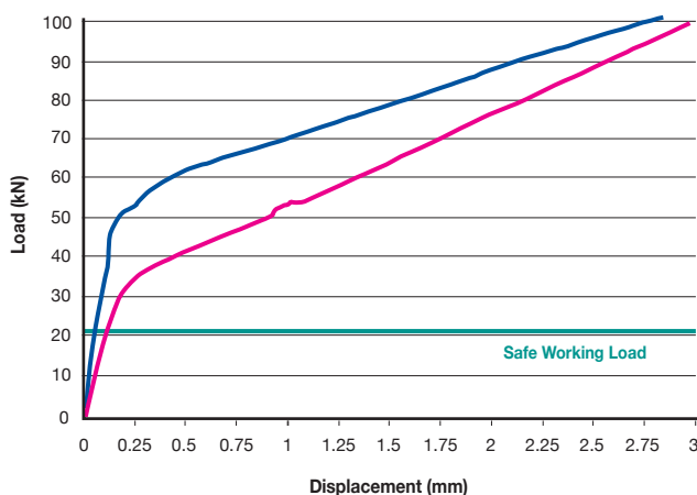
M16 - Connection Load vs Ply Displacement
