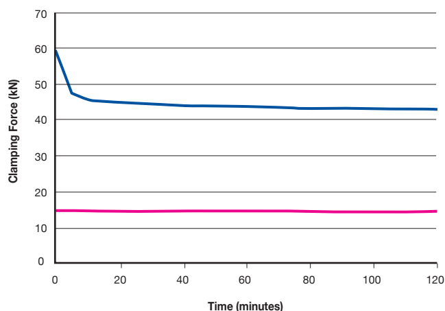
M16: Up to 3x Clamping Force
